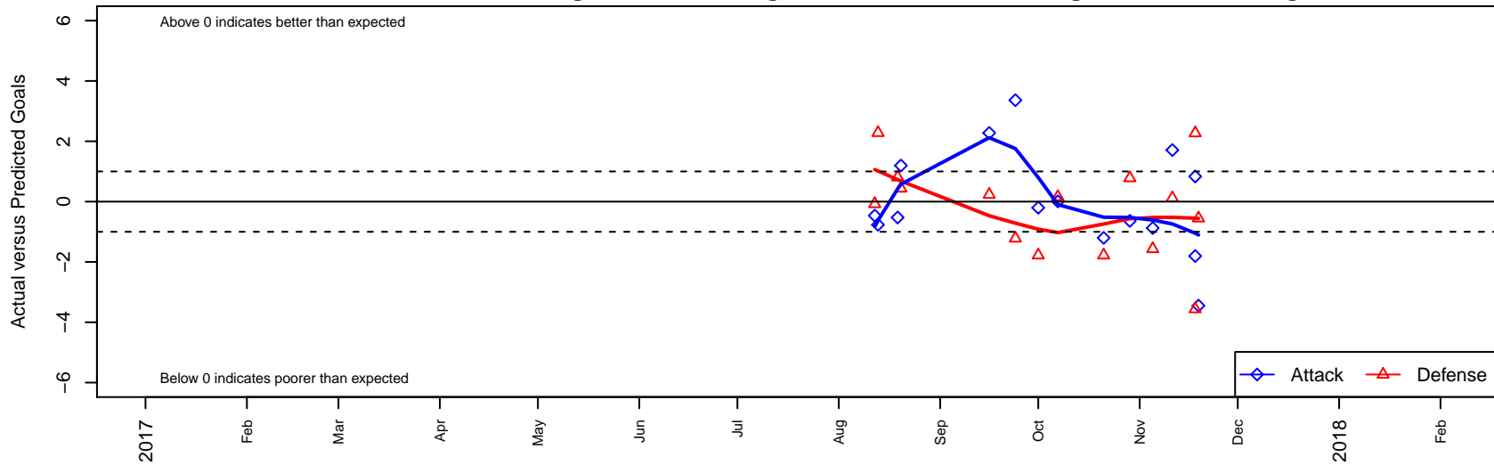
WA East G03 Dots are actual minus expected GF (blue circles) and GA (red triangles). Blue line is smoothed change in attack strength. Red is smoothed change in defense strength.
